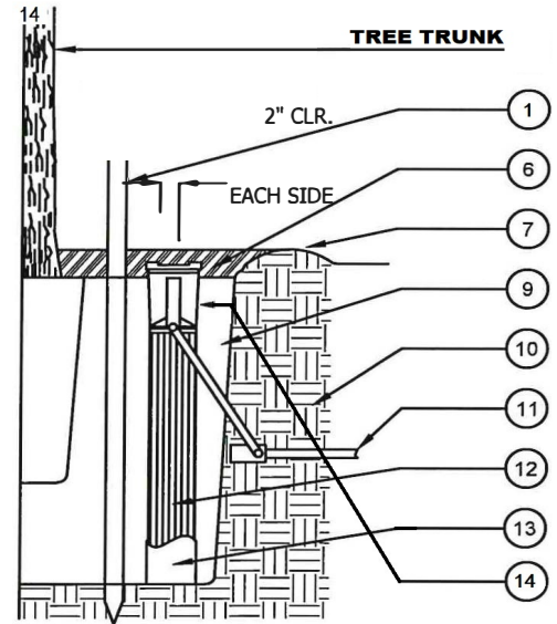
DETAIL 1
