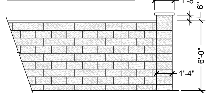
WALL: W-01 PILASTER: W-02, W-03 6'-0" TALL SPLIT-FACE BLOCK WALL W/ PRECISION BLOCK CAP
