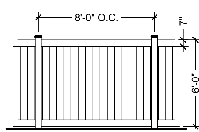
FENCE: W-04 6'-0" TALL INTERIOR VINYL FENCE, COLOR WHITE
