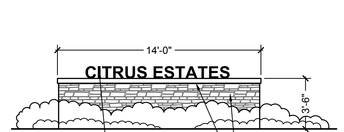
WALL: W-08 42" TALL ENTRY MONUMENT WALL PIN SET LETTERING STONE VENEER WALL PRECISION CAP
