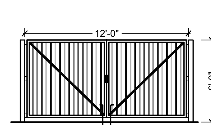
GATE: W-07 6'-0" TALL TUBULAR STEEL MAINTENANCE GATE
