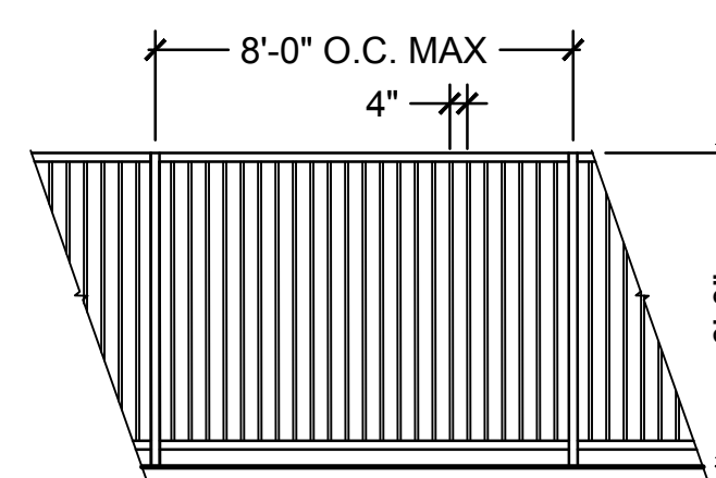
FENCE: W-06 6'-0" TALL TUBULAR STEEL VIEW FENCE
