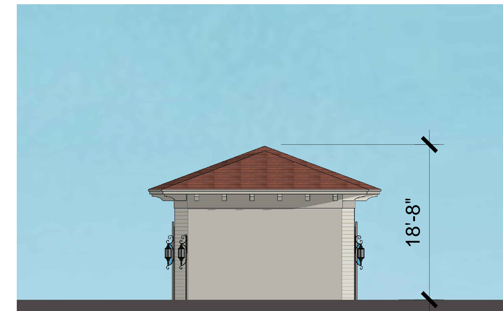
SOUTH ELEVATION
