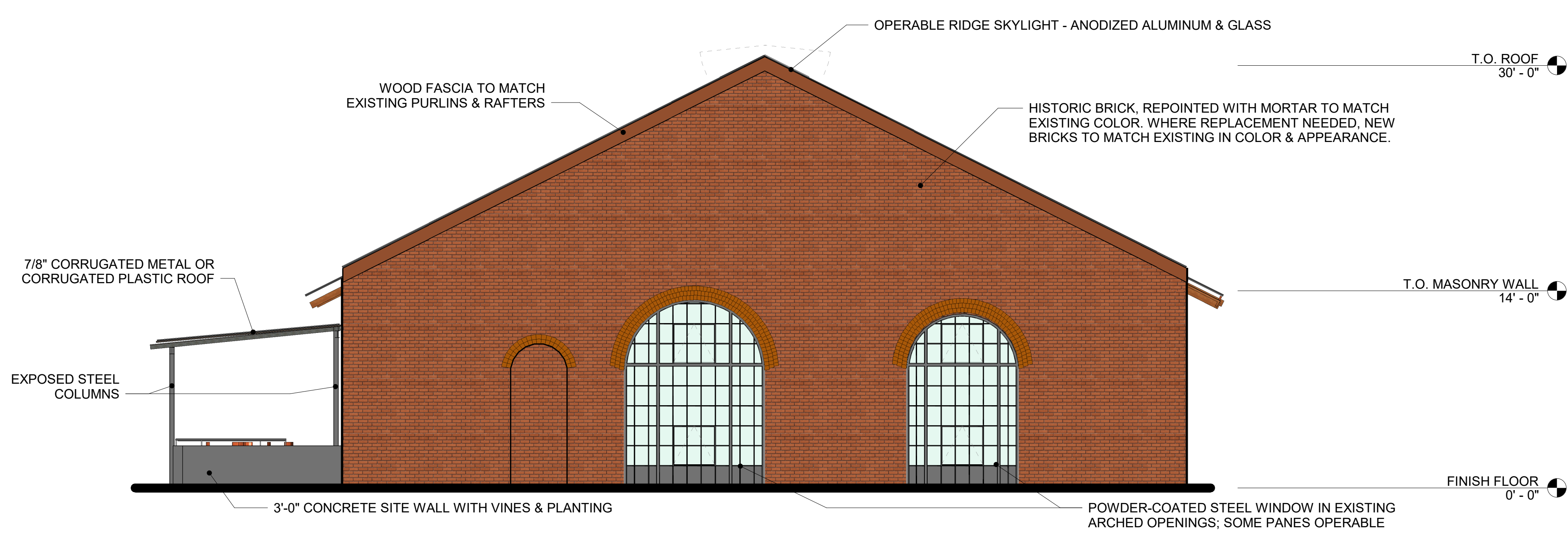
1 NORTH ELEVATION CUP-2 3/16" = 1'-0"
