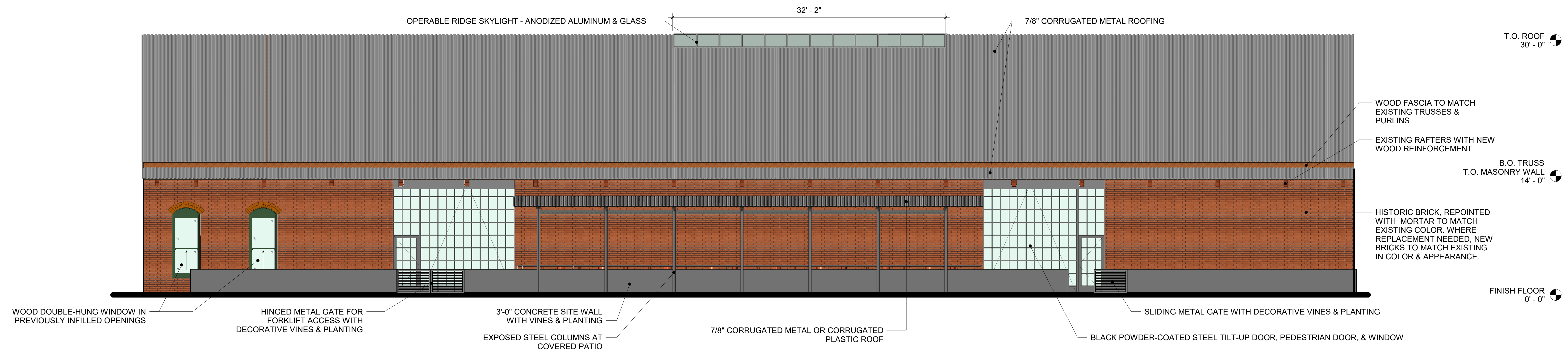
3 EAST ELEVATION CUP-2 3/16" = 1'-0"
