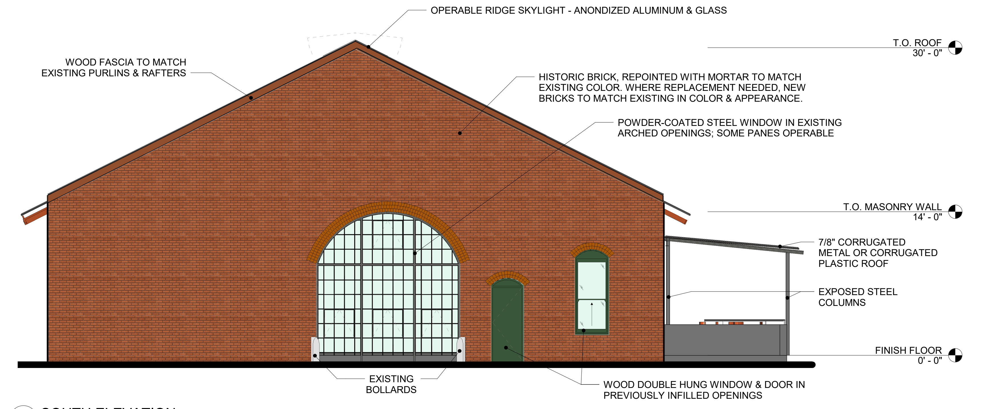
2 SOUTH ELEVATION CUP-2 3/16" = 1'-0"
