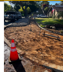
Contractor setting forms for sidewalk and ADA Ramp at the corner of Cimarron Dr. and Cimarron Ct.
